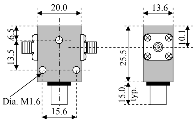
Units: mm Not to scale
