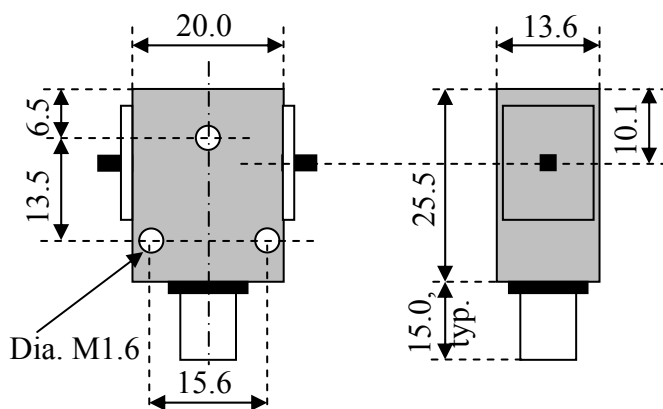
Optional – Input/Output pin: Ø=9mm, Length=3.0mm
