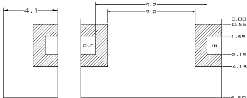
BOTTOM VIEW
